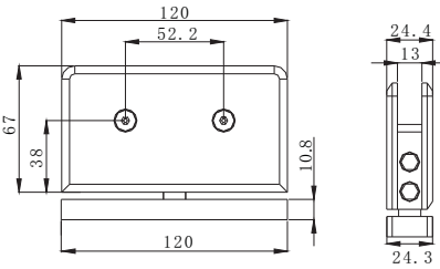
Top or Bottom Mount
