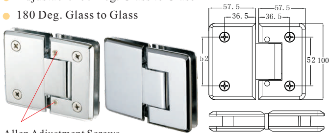
Allen Adjustment Screws
